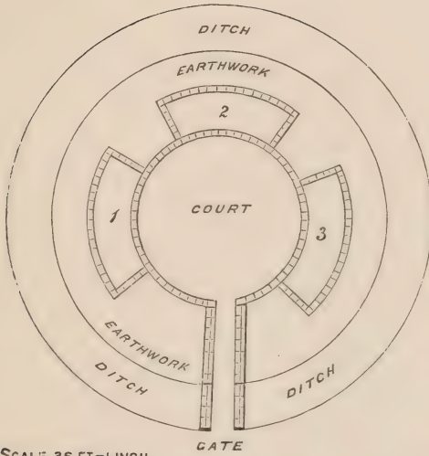
PLAN OF SMALL CIRCULAR FORT AT MASINDI, WITH FIRE-PROOF ROOMS; DITCH LEFT UNFINISHED.
